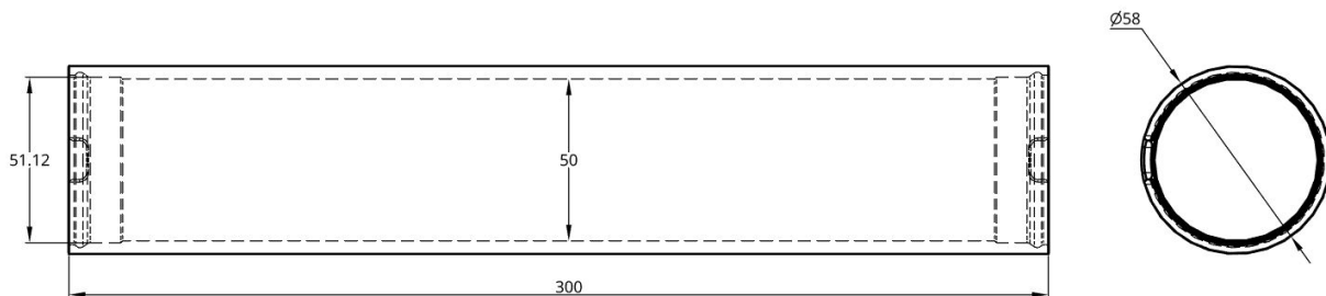
WTE2-M-LOCKING-TUBE-300-R1
