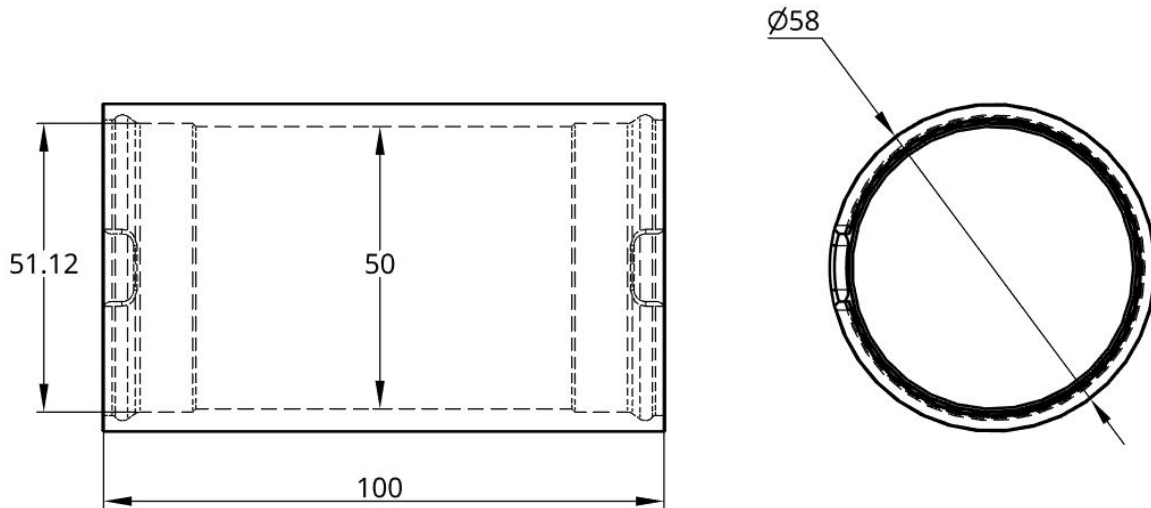
WTE2-M-LOCKING-TUBE-100-R1
